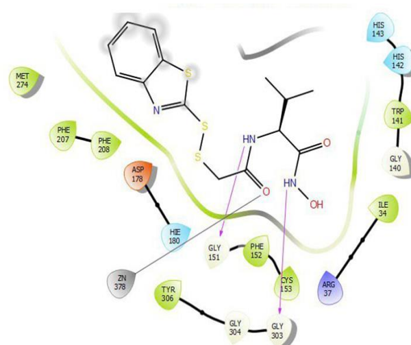
Figure 8: Docking of the hybrid 5 on HDAC8 type 1T69 protein
