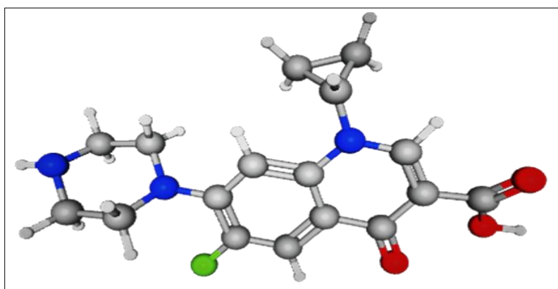
Figure 1: Ciprofloxacin's chemical structure
